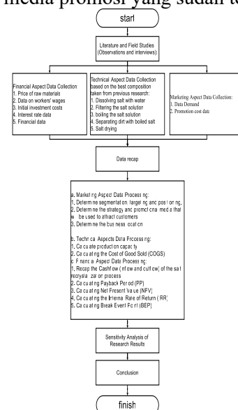
Gambar 2.2 Flowchart penelitian
