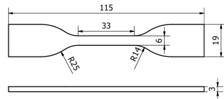
Gambar 3. Spesimen Benda Uji Standard Ukuran ASTM D638 type IV
