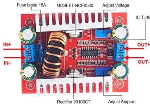
Gambar 8. DC-DC Step Up Converter 400W
