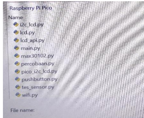
Gambar 2.2 Program Software
