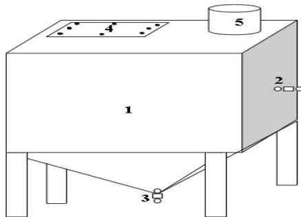
Gambar 2.4 Filter Asap
